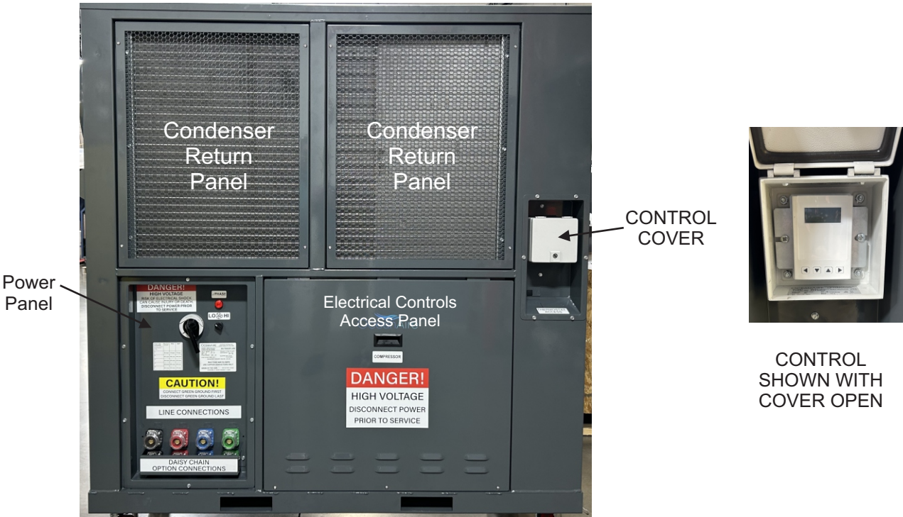
OPAC144 ELECTRICALS
