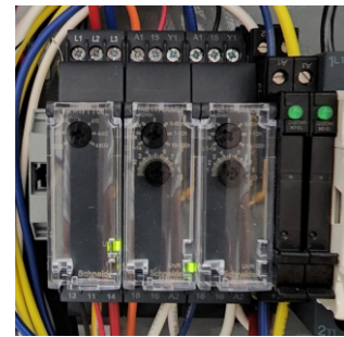
PHASE MONITOR - DISABLED (ONLY ONE LED ILLUMINATED)
