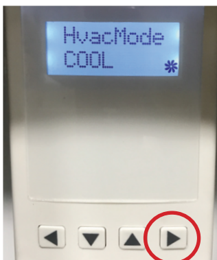
5. MODE Selection - Press Arrow Button
