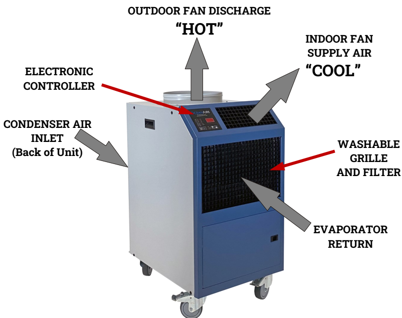
2OACH1211—COOLING MODE
