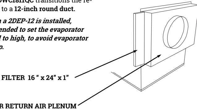
2DEP-12 EVAPORATOR RETURN AIR PLENUM for Ducting Return Air
